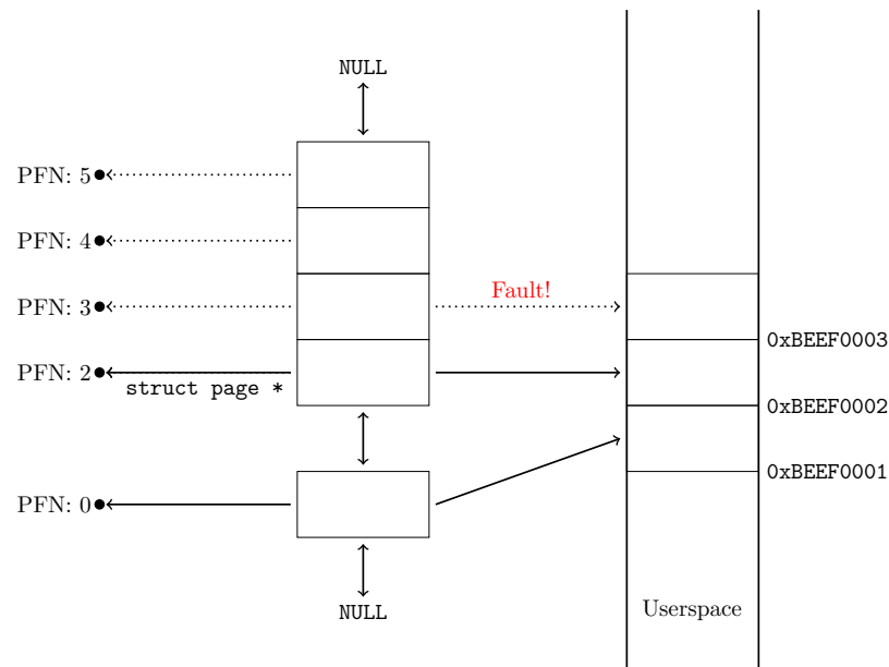
Figure 2.1: Misaligned Kernel Page Remap. Left column represents physical memory (addressed by PFN); center column represents in-module accounting of allocations; right column represents process address space.
