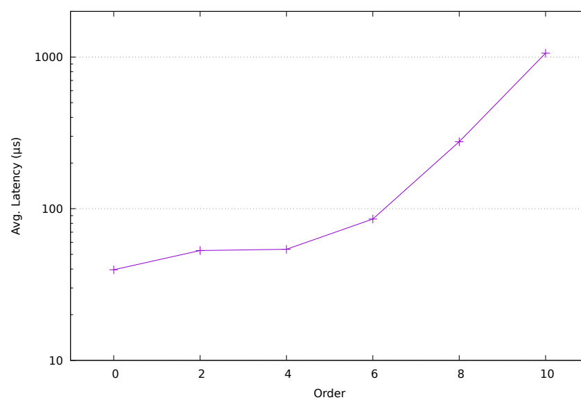
Figure 3.4: Average coherency op latency of variable-order contiguous allocation
